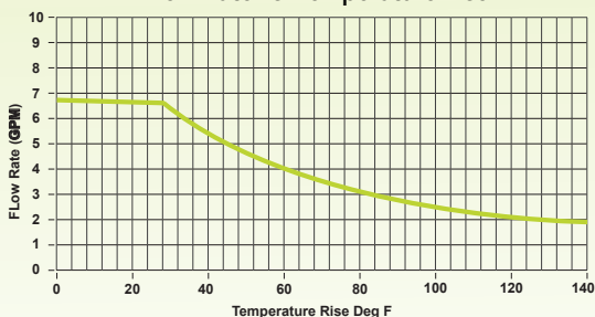
Flow Rate vs. Temperature Rise
